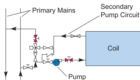
Primary-Secondary Connections
