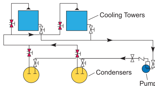
Cooling Tower & Chiller Connections
