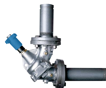
Flanged Model CBVA showing 90° angle installation.
